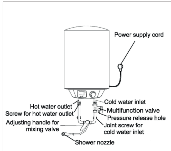
TYPICAL SINGLE OUTLET CONNECTION (Fig.3)
